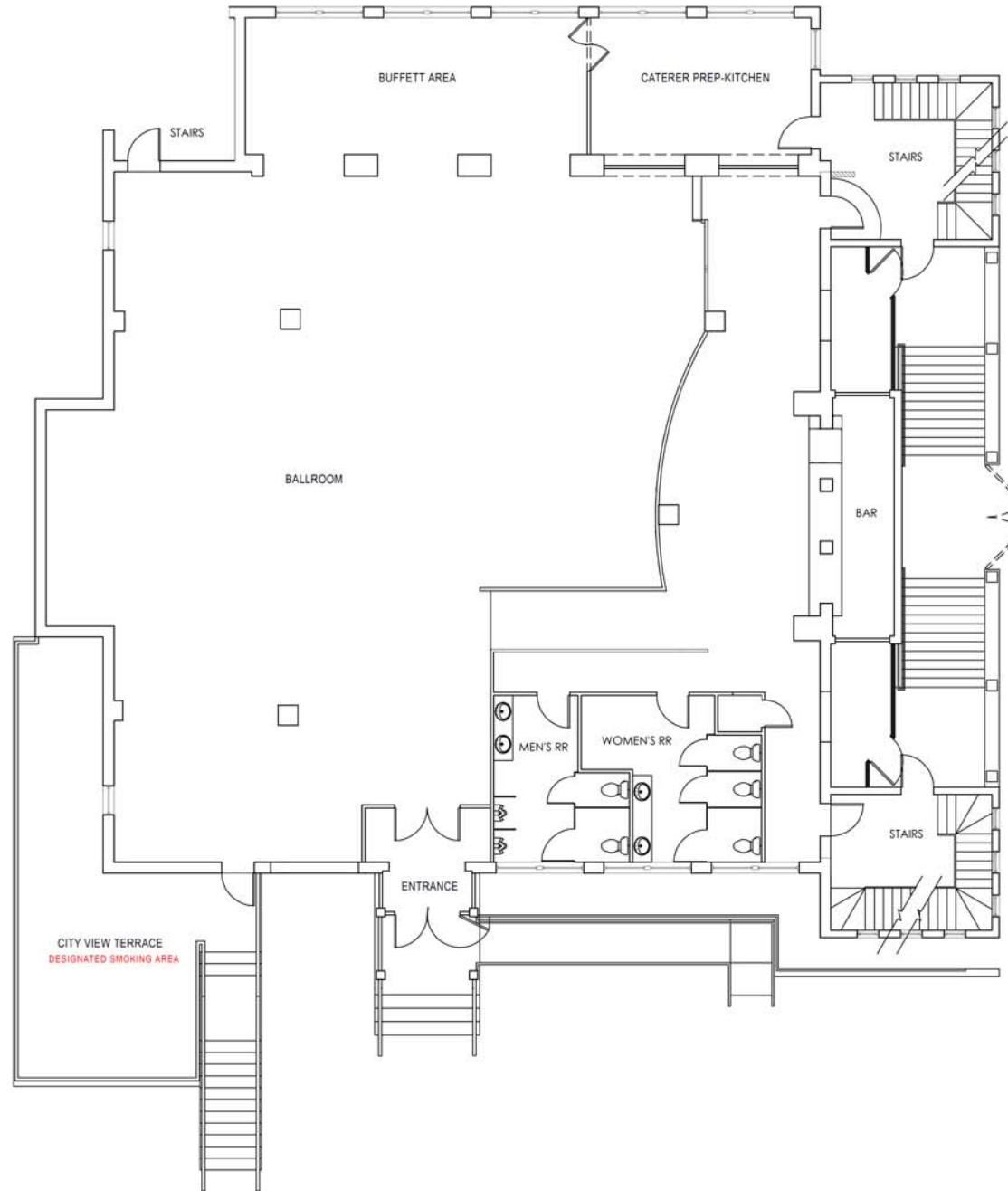
02 BALLROOM LEVEL & CITY VIEW TERRACE FLOOR PLAN A1.3 1/4"=1'-0"
